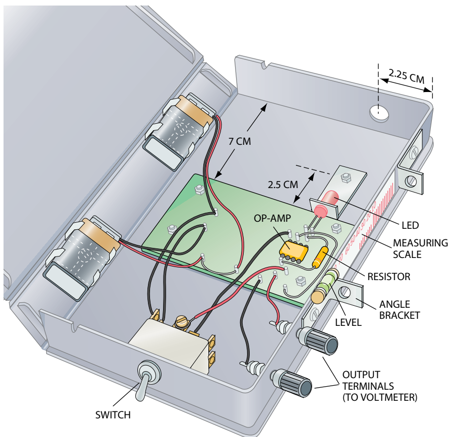
HAZE SENSOR
