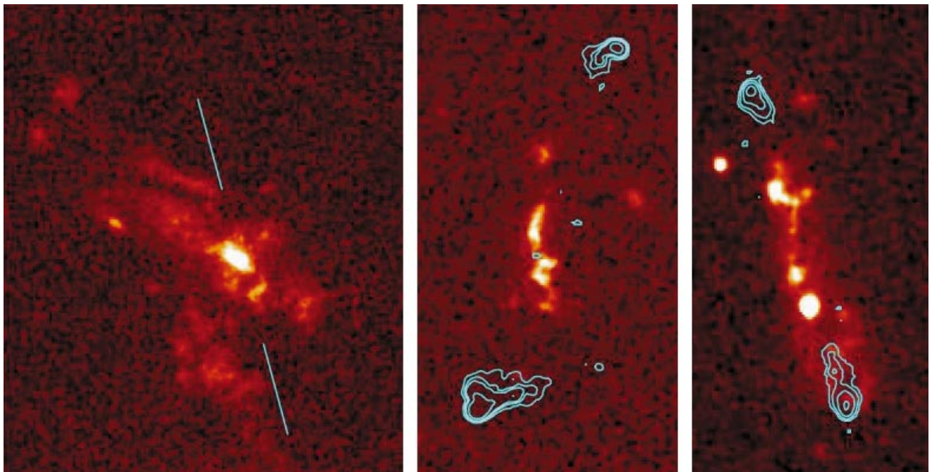
RADIO GALAXIES 3C265 ( left ), 3C324 ( center ) and 3C368 ( right ) exhibit unique morphological and spectral traits. For these composite images, the Hubble Space Telescope captured the galaxies ( red emissions ), and the Very Large Array Radio In-
