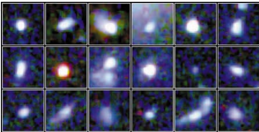
FAINT BLUE SUBGALACTIC CLUMPS , some 11 billion light-years from the earth, may well be the stuff from which today's galaxies were made. The Hubble telescope found these 18 objects in the northern part of the constellation Hercules, near Draco. Astronomers believe such small clumps collided and merged with one another to generate giant modern-day galaxies.
