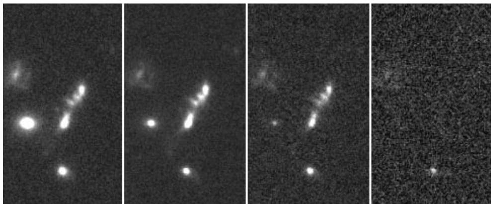
ULTRAVIOLET DROPOUT GALAXIES are common in the deepest astronomical images. Viewed through several filters, these distant galaxies are visible at blue, red and green wavelengths but disappear in near-ultraviolet images ( above ). Hydrogen, which is ubiquitous in galaxies and the spaces between them, absorbs all UV light that is bluer than a certain wavelength.
