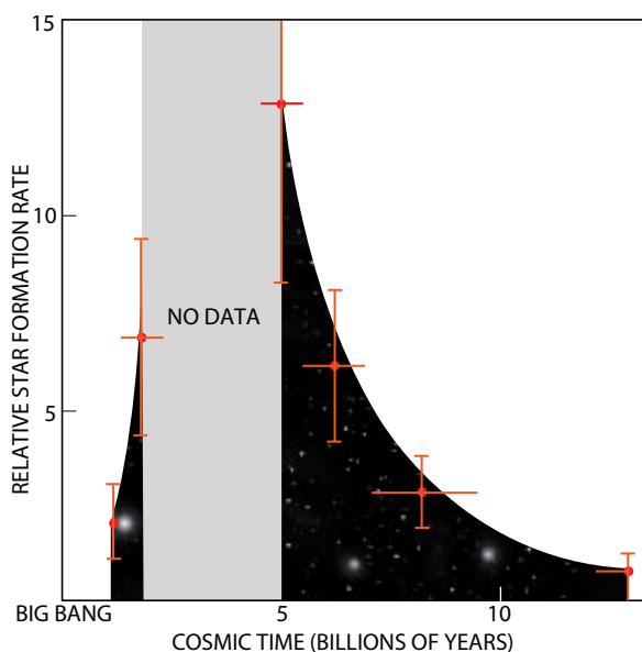
STAR FORMATION was swift 12 billion years ago when the universe was young, as shown on this graph, based on observations of distant galaxies using the Hubble telescope and earthbound telescopes. About nine billion years ago, the star formation rate—for reasons yet to be discovered—began to decline dramatically.
